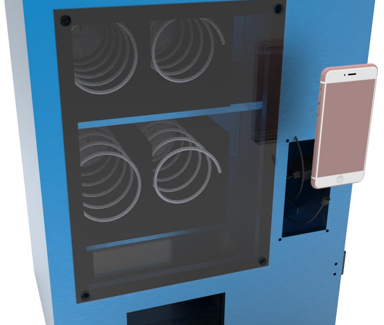
Smartphone is connected with charger which is charged via solar panel and power backup, the smartphone controls micro controller of the vending machine
